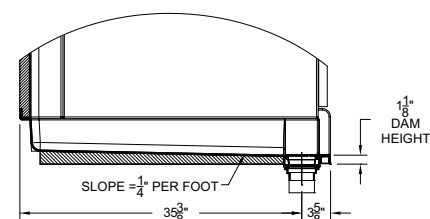
DETAIL VIEW
