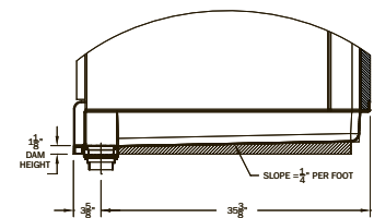
DETAIL VIEW
