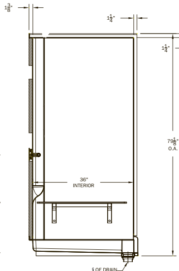
SECTION A-A SIDE VIEW
