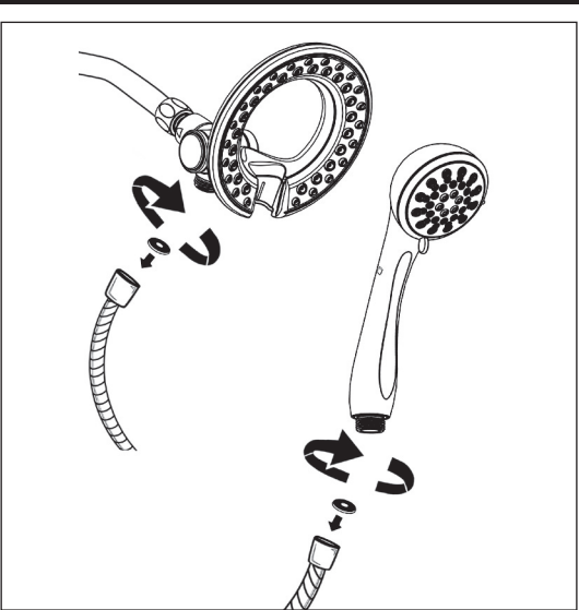
Flexible Hose
