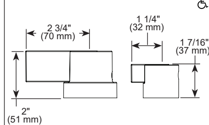
HL75P34-▲ Lever Handle
