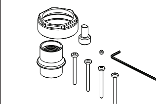
RP100160▲ Available Thick Wall Installation Kit
