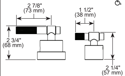
HL75P39-▲ Wire Handle
