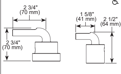
RP100160▲ Available Thick Wall Installation Kit
