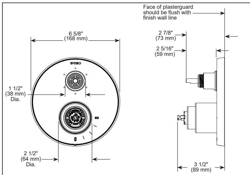
HL75P32-▲ Lever Handle
