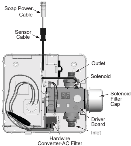
Hardwire Operated Control Box
