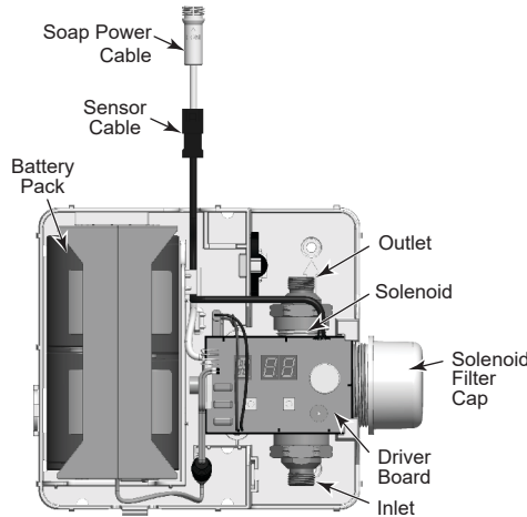
Battery Operated Control Box
