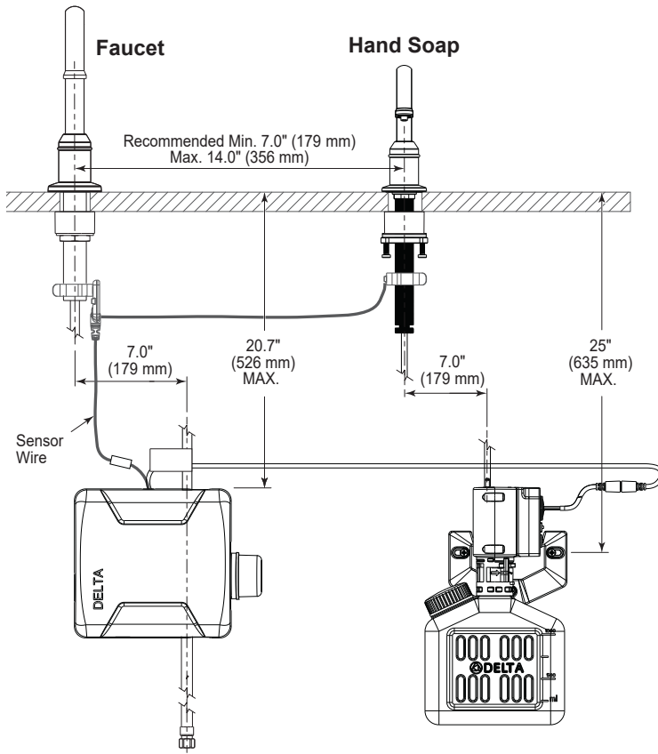
Hardwire Operated Control Box
