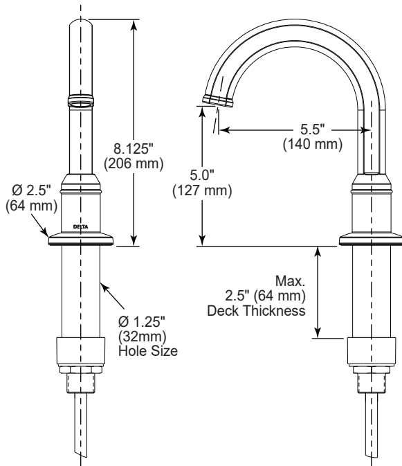
Single Hole Faucet without Black Spacer
