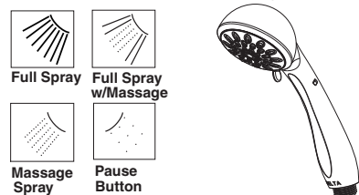
RP64025 ▲ Touch-Clean® 4-Setting Handshower
