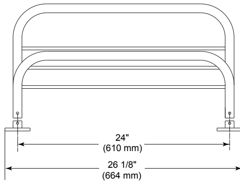
Mounting Specification
