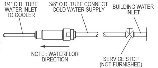
WALL ROUGH-IN
