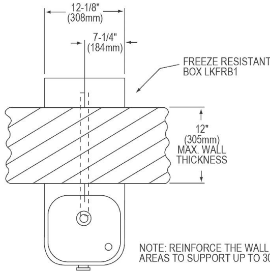
WALL ROUGH-IN
