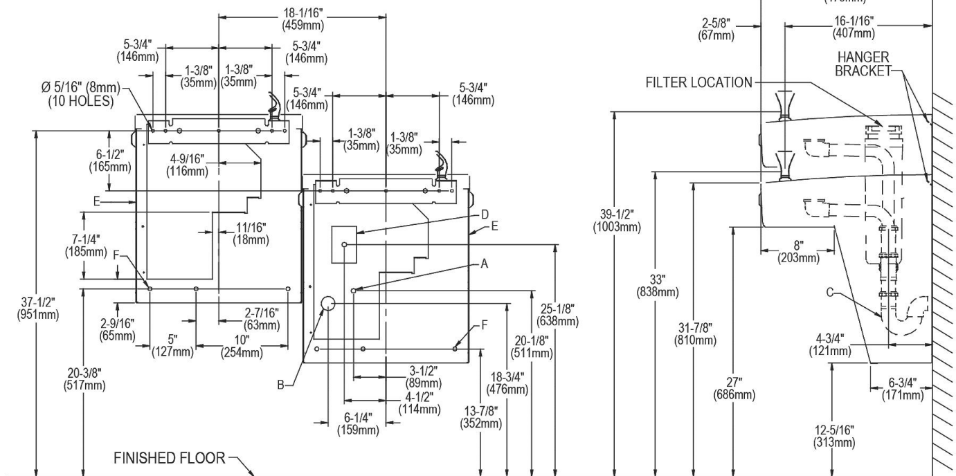
WaterSentry® VII Filter System
