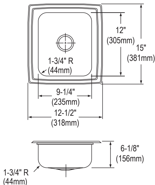
Model BPSFR1215 Illustrated
