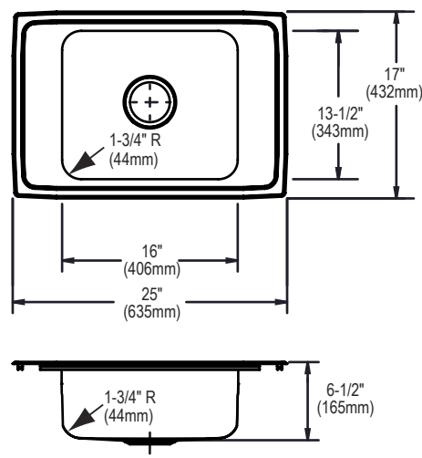
Model PSDKAD(Q)251765C Illustrated
