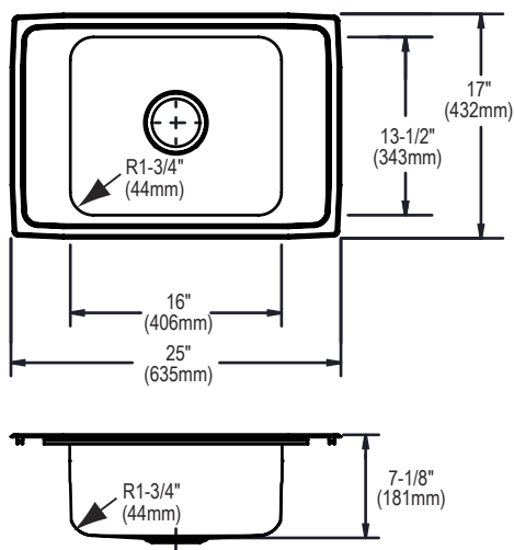
Model PSDKR(Q)2517 Illustrated
