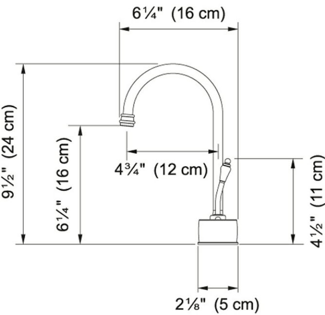
Technical Drawing
