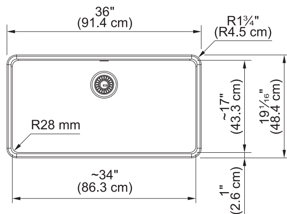
Dimensional Drawing
