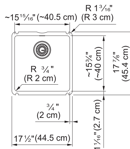
Dimensional Drawing
