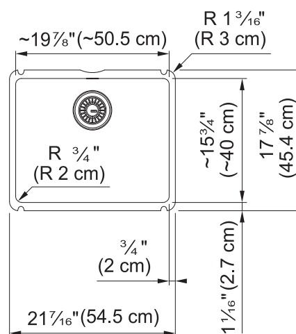
Dimensional Drawing
