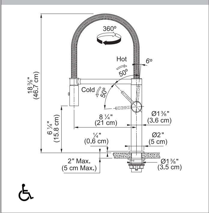
Dimensional Drawing
