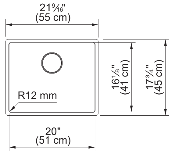
Dimensional Drawing
