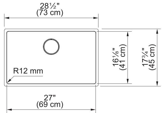
Dimensional Drawing
