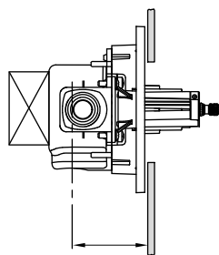
Pared delgada
