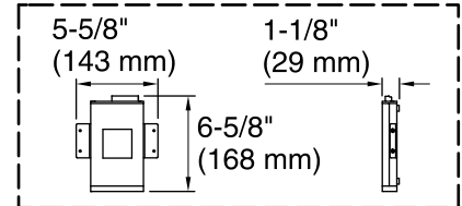
Amplifier
