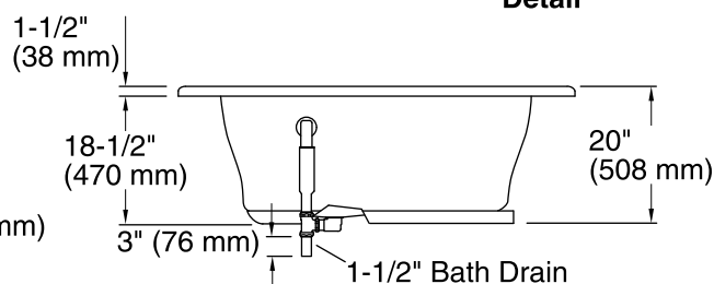
Drop-in Rim Detail
