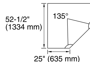
Drop-in Cut-out Detail
