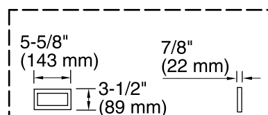
User Interface
