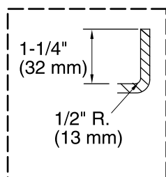
Flange Detail
