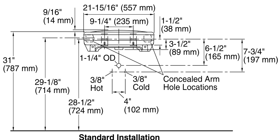
Standard Installation
