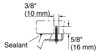
Sealant Wood Installation
