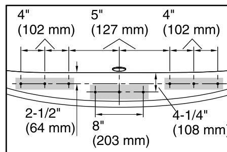
Faucet Hole Location (For KOHLER® Brand Only)
