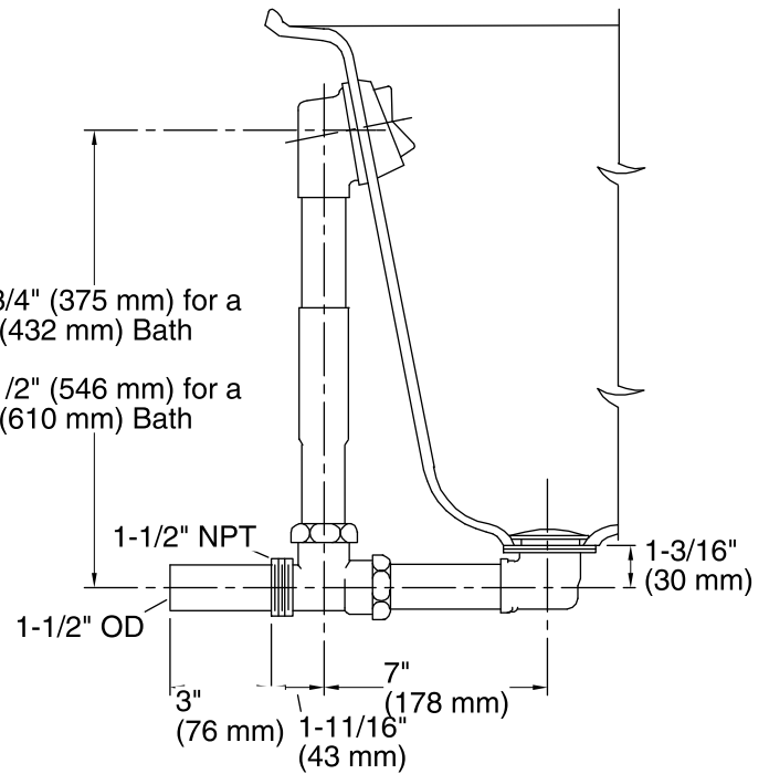
Above-the-Floor
