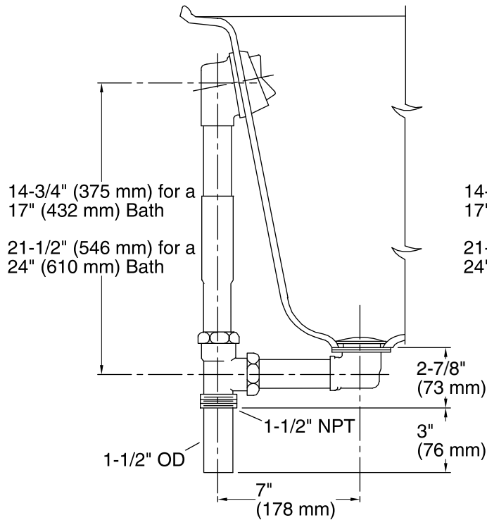
Through-the-Floor
