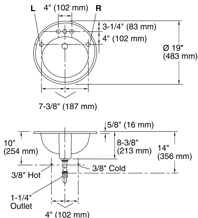
Standard Installation
