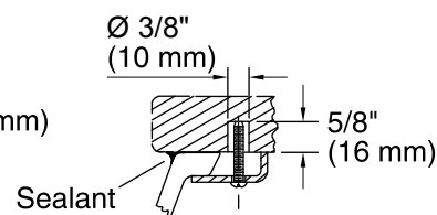
Marble Installation
