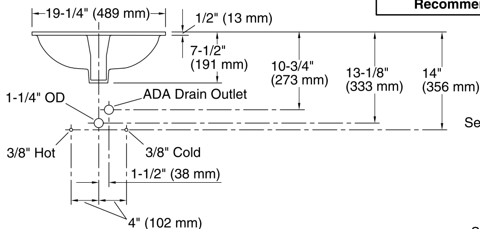
Standard Installation
