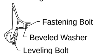
Leg Detail
