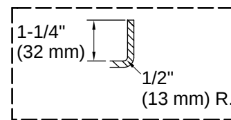
Integral Flange Detail
