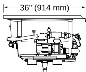
1-1/2" Bath Drain
