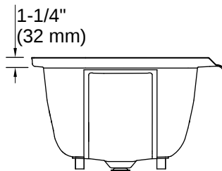
1-1/2" Bath Drain
