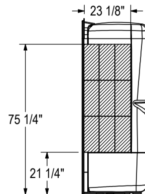
OPTIONNAL REINFORCEMENT (Left shown, Right symmetrical)
