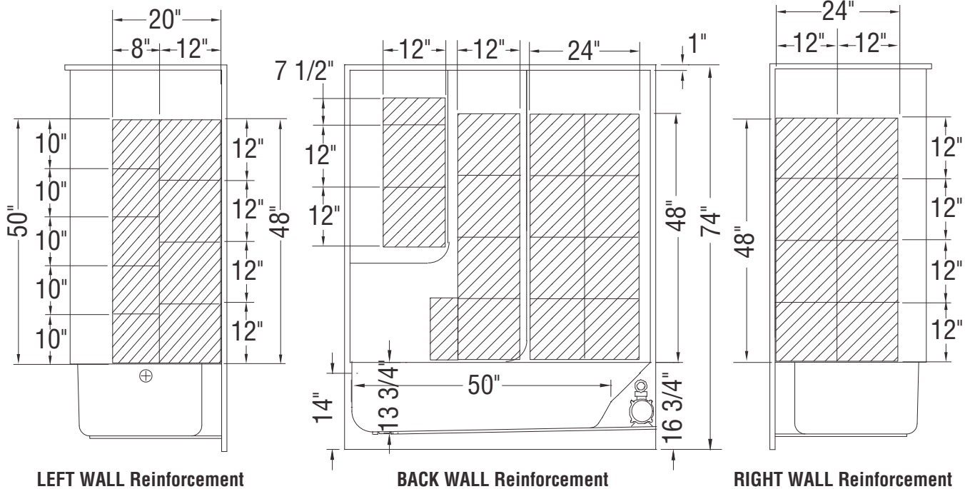
Full Wall Reinforcement Shown
