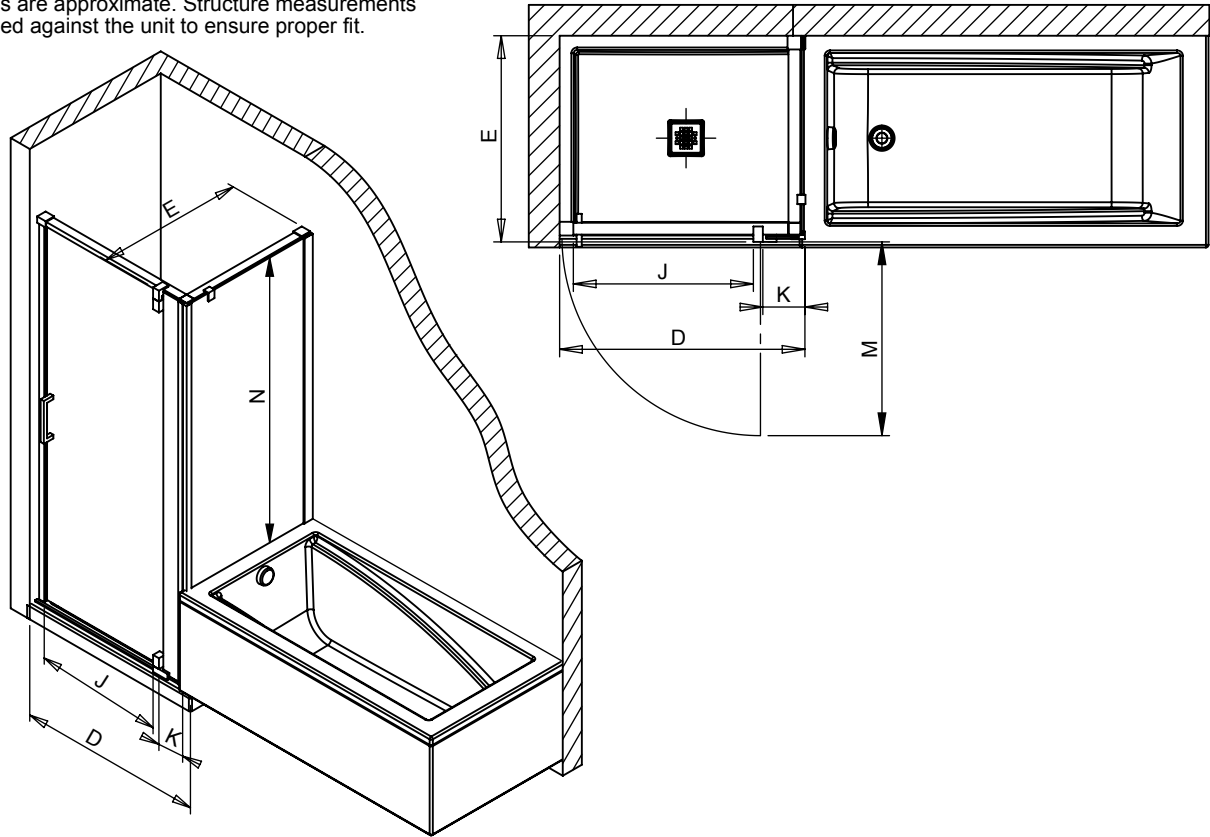
CLOSED ON BATH (LEFT OR RIGHT)
