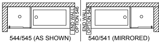
CLOSED ON PANEL (LEFT OR RIGHT)
