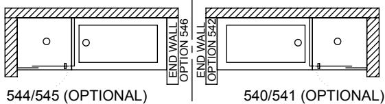
CLOSED ON BATH (LEFT OR RIGHT)
