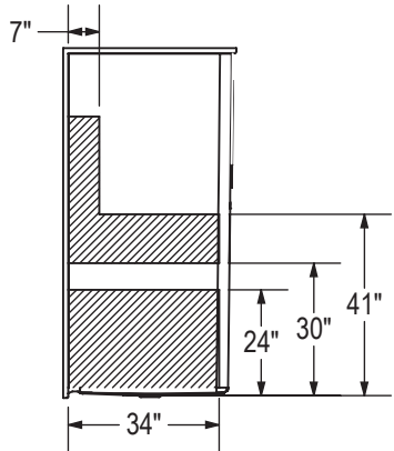
RIGHT WALL SHOWN LEFT WALL SYMMETRICAL
