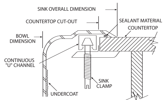
Installation Detail
