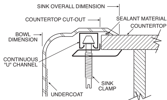
Installation Detail
