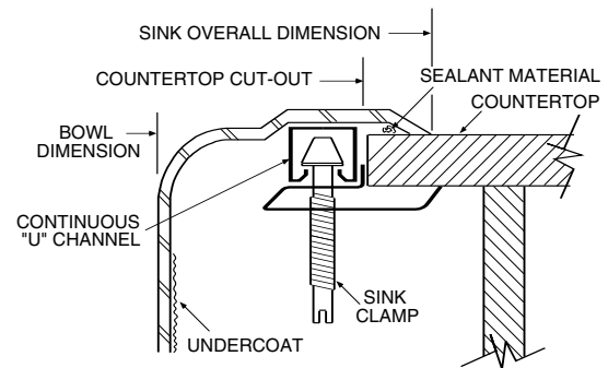
Installation Detail
