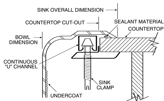
Installation Detail
