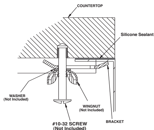
Installation Detail
