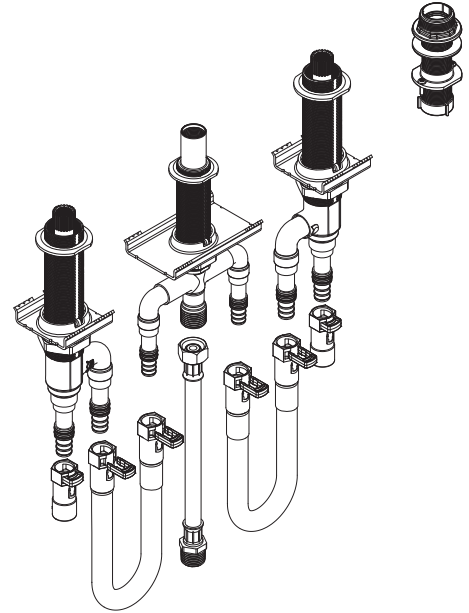
Roman Tub High Flow Rough-In Valve (Adjustable Type)
