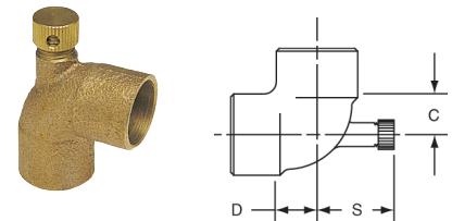
705-D ⚠ Vent Elbow C x C - Cast
