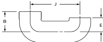
875-S ⚠ DWV Trap Upturn M x S – Cast
