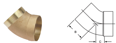
806-2 ⚠ DWV 45° Fitting Elbow Ftg x C – Cast
