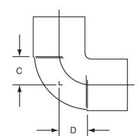
607 90° Elbow – Close Rough C x C – Wrot
