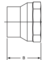
903-2 DWV Fitting Adapter Ftg x F – Wrot
