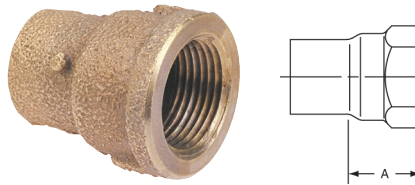
703 ▲ Adapter C x F – Cast
