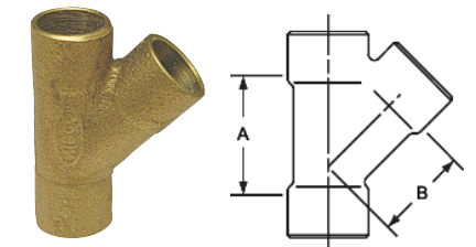
749 ⚠ 45° Y C x C x C – Cast
