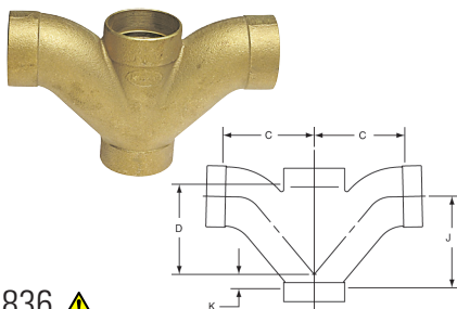
836 ⚠ DWV Double Long Turn T-Y C x C x C x C – Cast
