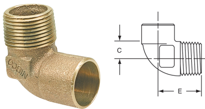
707-4 ⚠ 90° Elbow C x M – Cast
