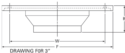
DRAWING FOR 3"
