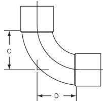
607-I 90° Elbow – Intermediate Radius C x C – Wrot
