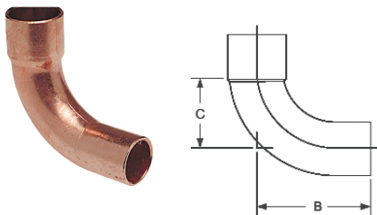
607-2-LT 90° Fitting Elbow – Long Radius Ftg x C – Wrot
