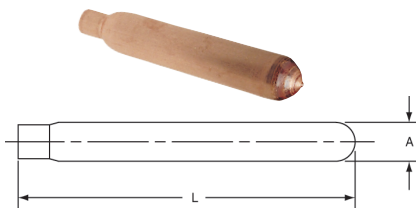
619 Air Chamber Ftg. – Wrot
