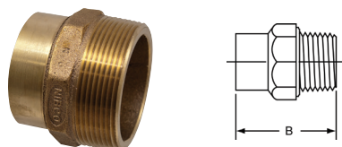
804-2 DWV Fitting Adapter Ftg x M – Cast
