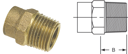
704 ⚠ Adapter C x M – Cast
