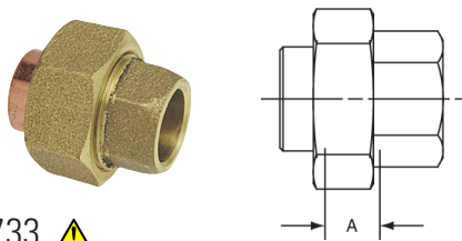
733 ⚠ Union C x C – Cast
