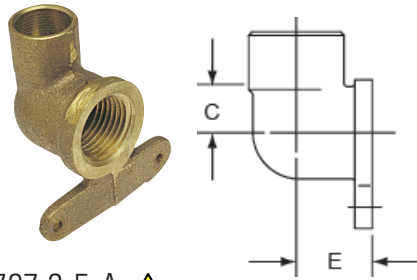
707-3-5-A ⚠ 90° Hy-Set Elbow C x F – Cast
