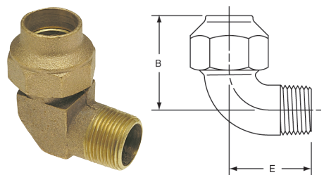
507-4 ⚠ Flared 90° Elbow FL x M – Cast
