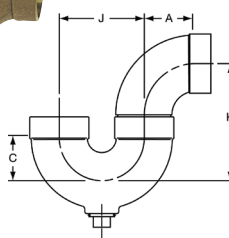
884 ⚠ DWV P-Trap w/Cleanout C x C x Cleanout w/Plug – Cast
