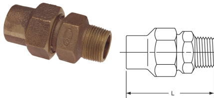
104 ⚠ Heavy Flared Adapter FL x M – Cast
