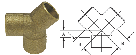
748 ⚠ 90° Y C x C x C – Cast
