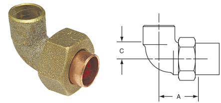
707-6 ⚠ 90° Union Elbow C x C – Cast
