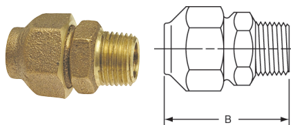
504 ⚠ Flared Adapter FL x M – Cast
