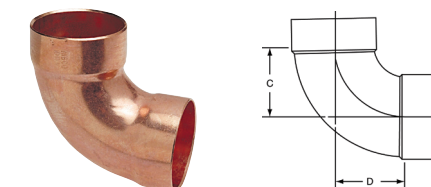
907 DWV 90° Elbow C x C – Wrot
