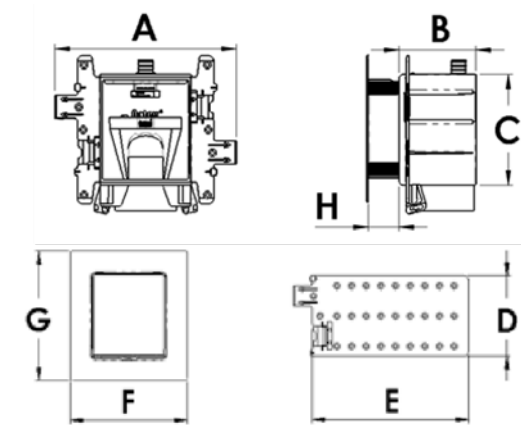
Quarter-Turn Drainage Funnel
