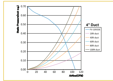
FV-10VS3E 4" Oval Duct
